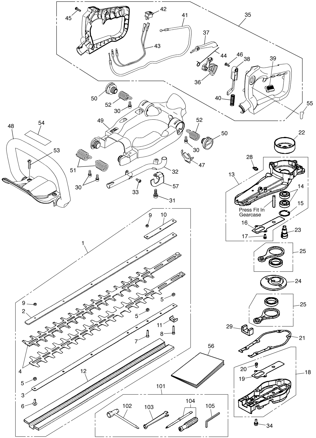
Fig.2 CUTTING UNIT CHTZ2400 (S/N 40100101 and up) CHTZ2400-L (S/N 40100101 and up)
